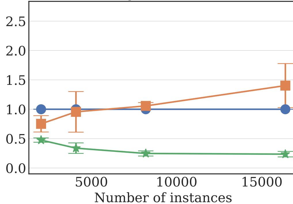
Synthetic 1
